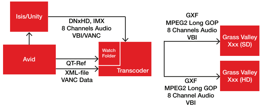
A post-to-broadcast transcoding workflow in which content from the NLE's SAN is converted for use on the broadcast servers of a station or network.
