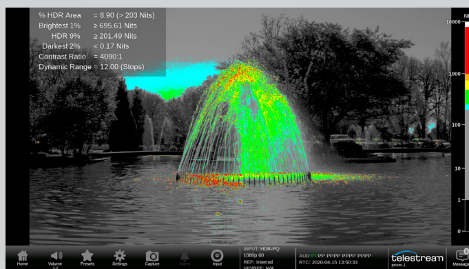
False color display to confirm with standards of brightness, percent HDR and dynamic range of the scene.
