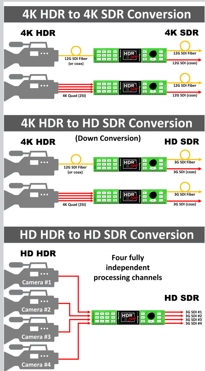
By installing different constellations (configuration of processing features) the greenMachine can be used for many different applications.
